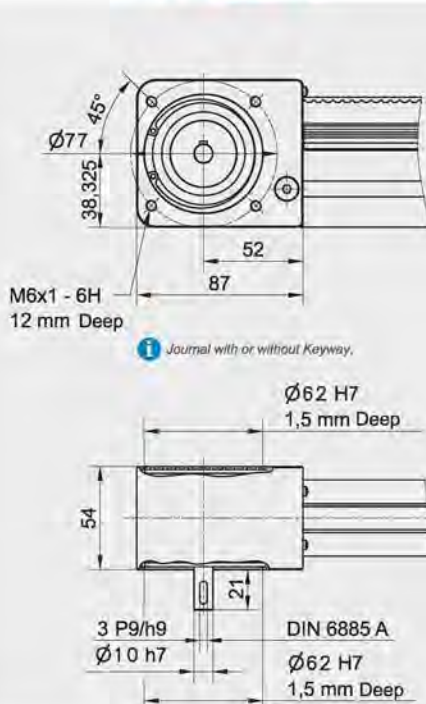
TYPE 1 L and 1 R
