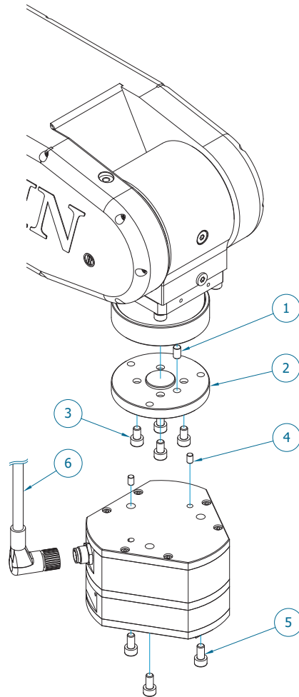
STG-16 & RA605 – Assembly explosion diagram
