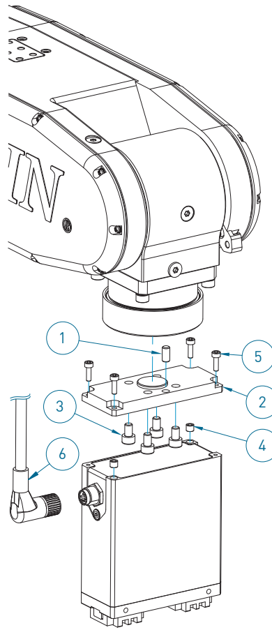
SEG-24 & RA605 – Assembly explosion diagram
