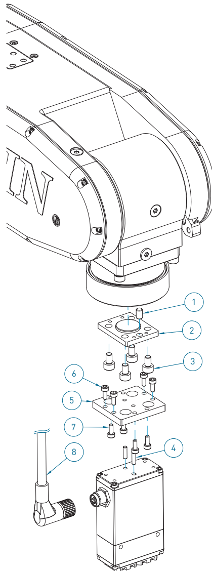
SEG-04 & RA605 – Assembly explosion diagram
