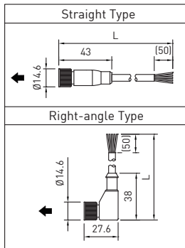
Connector Cable:
